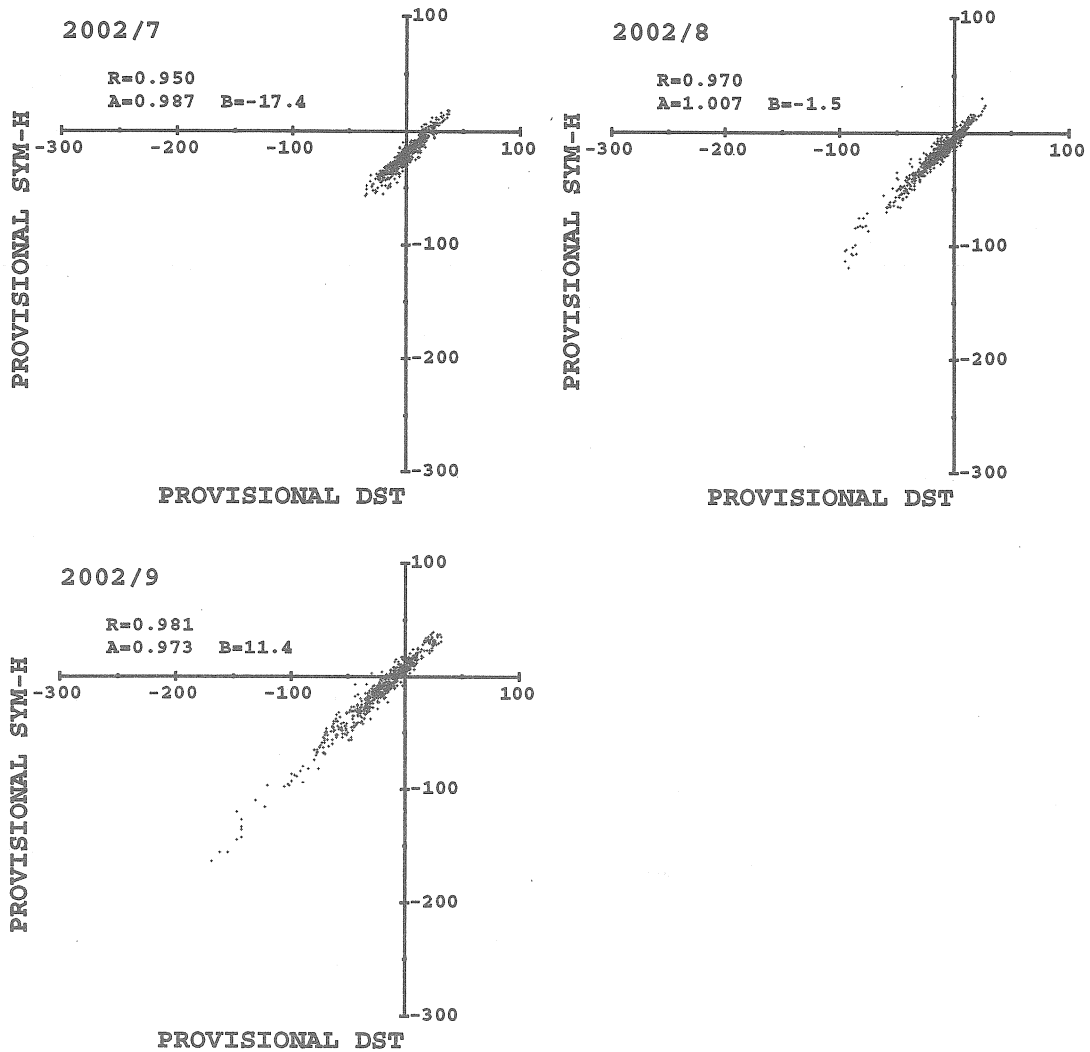
Figure 3b. Correlation plots for July-September, 2002. (Provisional Dst for October, November and December has not yet been available at the time of this publication.)
