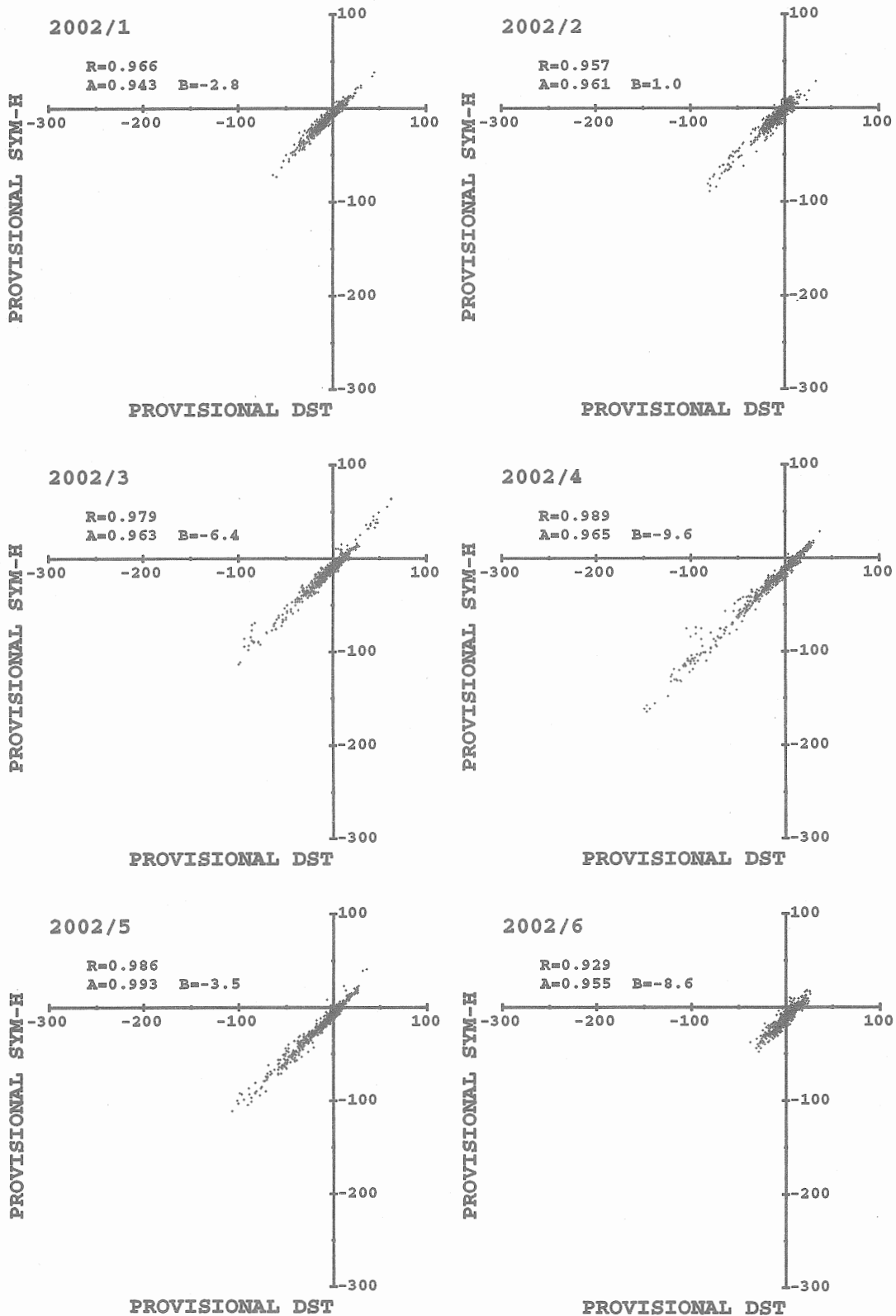
Figure 3a. Correlation plots between the hourly averaged SYM-H and the provisional Dst for January-June, 2002. The correlation coefficients R, the parameters of the regression line A and B (i.e. \text{SYM-H} = A \cdot \text{Dst} + B ) are shown on each panel.
